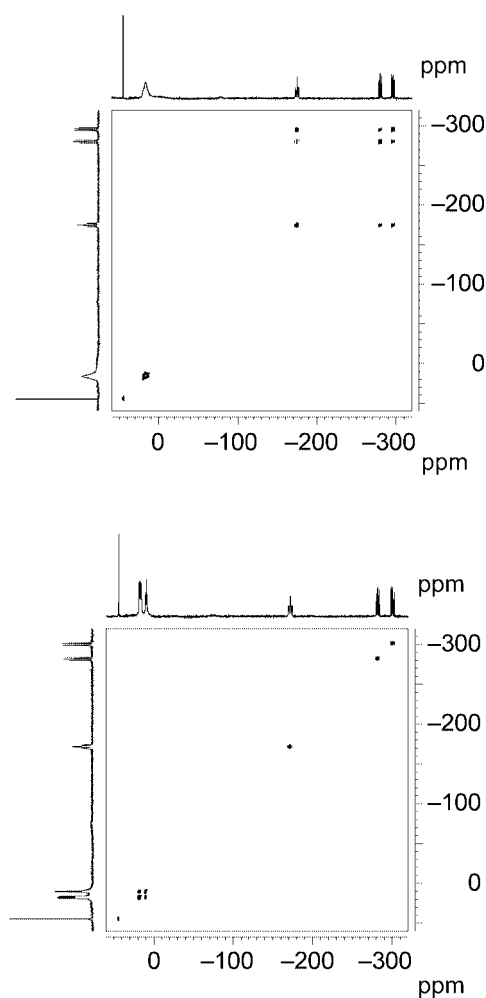
Figure 3. ^{31}\text{P}\{^1\text{H}\} EXSY spectra of 11 ( \text{CD}_2\text{Cl}_2 , 161.95 MHz, \tau_m 0.1 s). Top, spectrum at 294 K; bottom, spectrum at 248 K.
