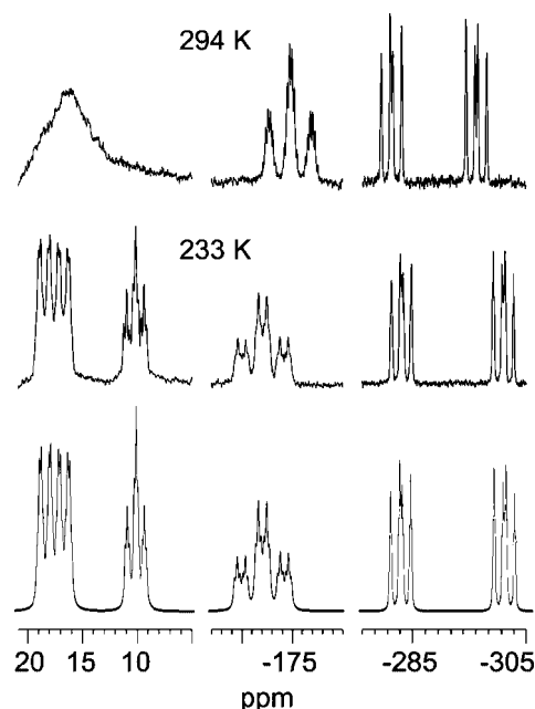
Figure 2. Sections of the ^{31}\text{P}\{^1\text{H}\} NMR spectra of 11 ( \text{CD}_2\text{Cl}_2 , 161.95 MHz). Top, experimental spectrum at 294 K; middle, experimental spectrum at 233 K; bottom, simulated spectrum at 233 K. The resonances due to the \text{PCy}_3 phosphorus are omitted for clarity.
