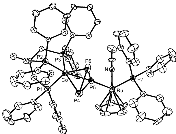
Figure 1. A view of the [(\text{triphos})\text{Co}](\mu, \eta^3\text{-P}_3)\{\text{CpRu}(\text{CH}_3\text{CN})(\text{PPh}_3)\}^+ cation in the structure of 6 ; displacement ellipsoids traced at the 20 % probability level. H atoms are not shown and labels for the carbon atoms are omitted for clarity.
